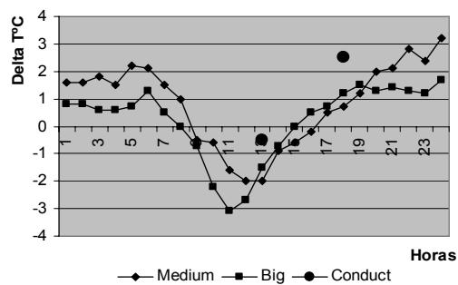
Figure 6: Comparison of air temperature in spaces connected to a big and medium courtyards and a conduct with respect to the local reference station data.
