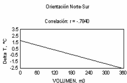
Figure 4: Differences of air temperature in rectangular inner patios with respect to local reference station data. Temperature tend to decrease when volume and height increases.
