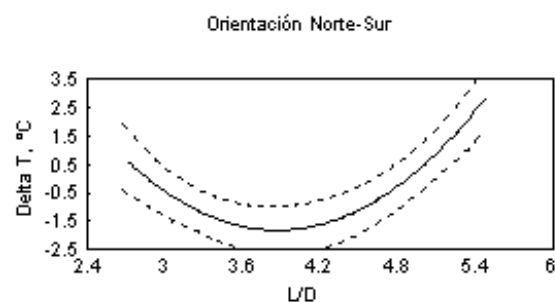
Figure 3: Differences of air temperature in rectangular inner patios with respect to local reference station data. Temperature tends to decrease with L/D=1:4.
