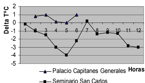
Figure 5: Differences of air temperature in patios with different quantity of vegetation, respect to the local reference station data; Capitanes Generales Palace, 35% and San Carlos Seminar, 80%.
