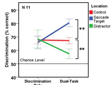
Figure 4. Discrimination performance at the three probed locations with (dual task) and without (discrimination only) eye movements in Experiment 1.
