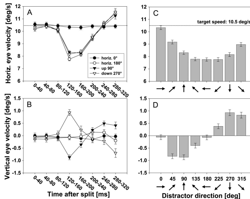
Figure 2. Mean horizontal and vertical eye velocity for tracking a horizontal target in Experiment 1 ( N = 14 ). The error bars represent the 95% confidence intervals of the means ( SE = 1.96 ). A: Horizontal eye velocity for cardinal distractor directions for time interval 0–320 ms after stimulus split. Solid circles denote the control condition, in which the distractor moved horizontally in the exact same direction as target. The dashed lines in Panels A and C denote target velocity ( 10.5^\circ/\text{s} ). B: Vertical eye velocity for cardinal distractor directions for time interval 0–320 ms. C: Horizontal eye velocity for all distractor directions averaged across time interval 120–160 ms after stimulus split. D: Vertical eye velocity for all distractor directions averaged across time interval 120–160 ms.
