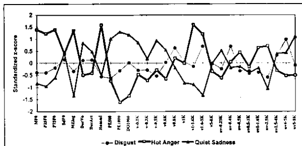
Figure 2. Acoustic profiles for three selected emotions. See contribution by Johnstone, Banse, & Scherer, this volume, for the legend of acoustic variables.
