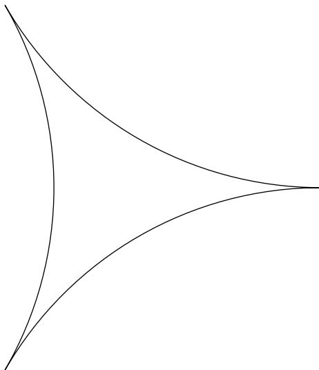
Figure 7. Un triangle D -fin.
