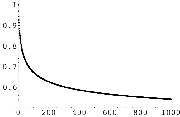
Figure 6. Coordinates of the eigenvector
