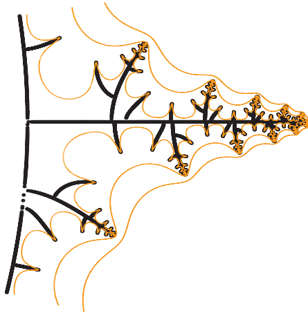
Figure 4. The image of a small boundary arc under \bar{f}_3 with three Green's lines.
