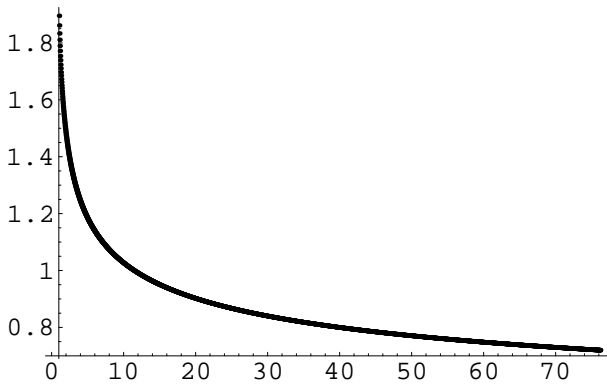
Figure 8. Values of I(r)
