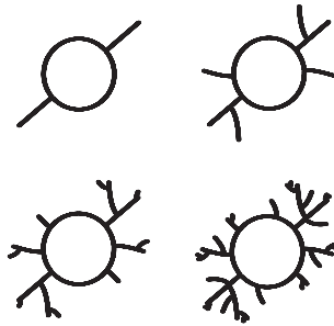
Figure 1. Images of \bar{f}_1, \bar{f}_2, \bar{f}_3, and \bar{f}_4
