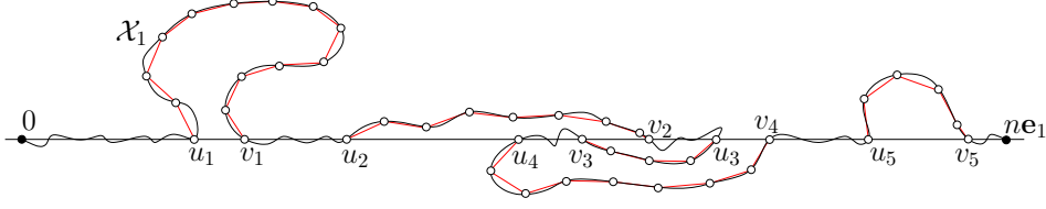
FIGURE 5. Coarse-graining the excursions of a path \pi : 0 \rightarrow ne_1 .
