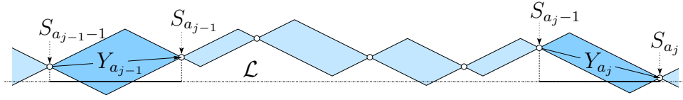
FIGURE 3. The proof of the upper bound: the size of the intersection of a diamond with \mathcal{L} is bounded above by the size of its projection on \mathcal{L} .
