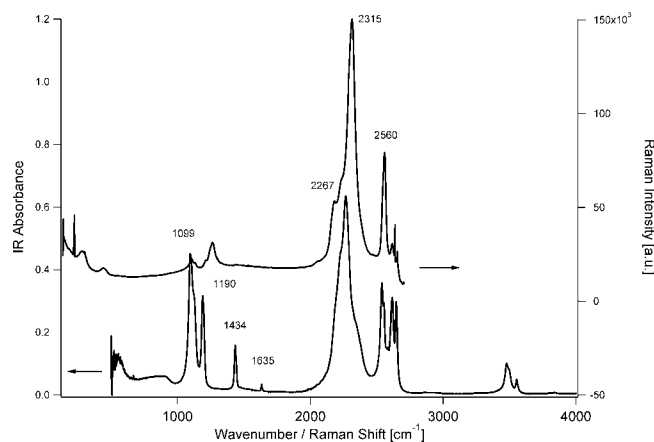
Figure 4. IR and Raman spectra of \text{NaBH}_4\cdot 2\text{D}_2\text{O} (95% D isotope purity) at room temperature.
