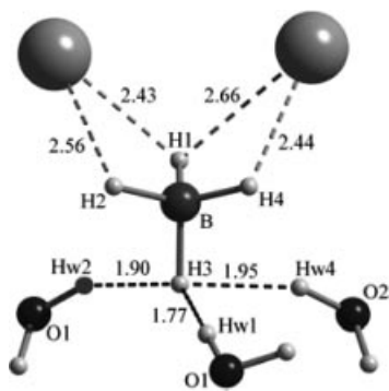
Figure 2. Coordination of the borohydride anion in \text{NaBH}_4 \cdot 2\text{H}_2\text{O} by two sodium atoms and three water molecules. Interatomic distances are shown in Å for the corrected hydrogen atom positions at 100 K.
