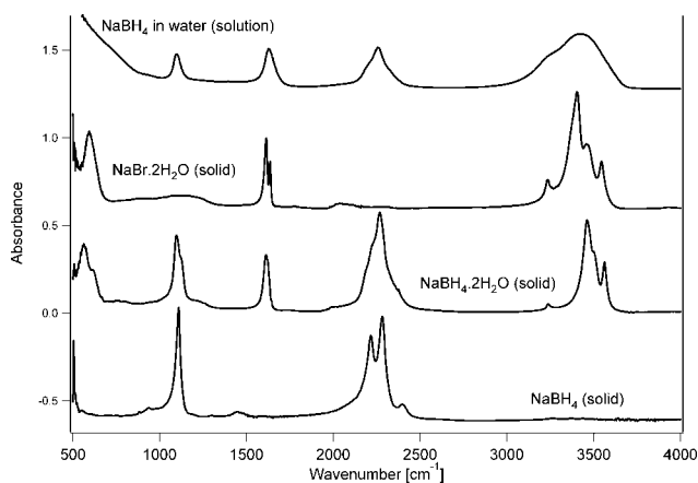
Figure 3. Room-temperature IR spectra of solid \text{NaBH}_4 , solid \text{NaBH}_4\cdot 2\text{H}_2\text{O} , solid \text{NaBr}\cdot 2\text{H}_2\text{O} and alkaline ( \text{pH} > 13 ) 8.8 M aqueous solution of \text{NaBH}_4 .
