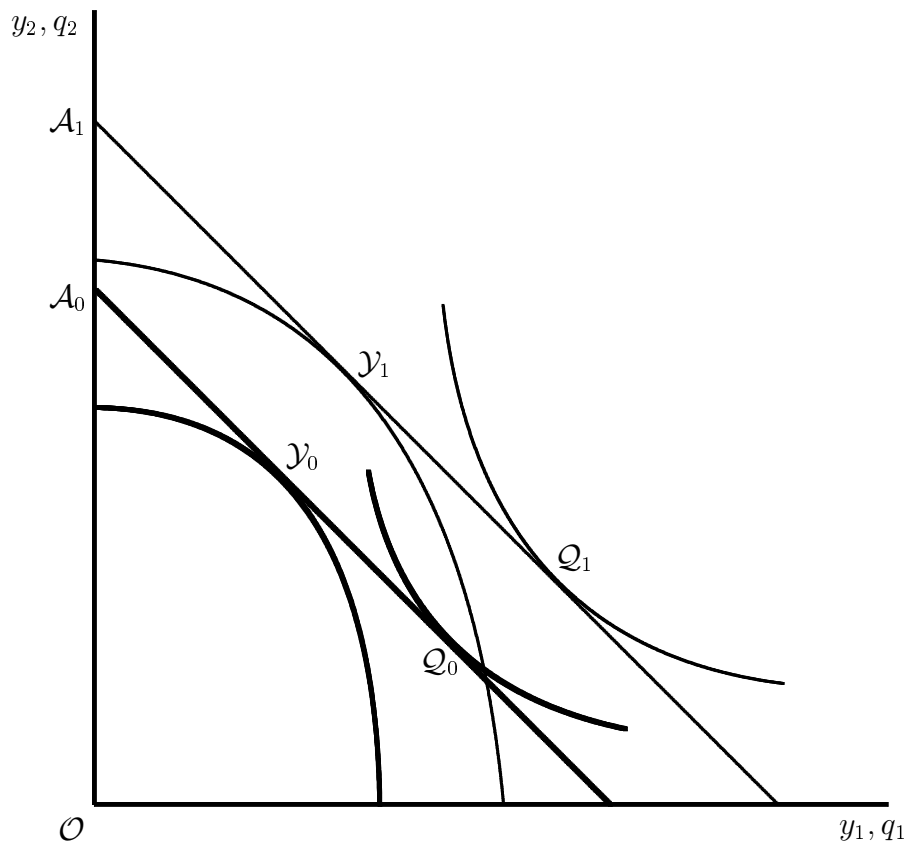
Figure 1: Endproducts Model — A technological improvement increases real GDP and real income (from OA_0 to OA_1 )
