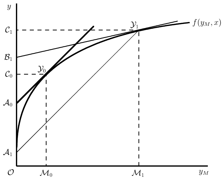
Figure 3: Middle-Products Model — An improvement in the terms of trade increases real income (from \mathcal{O}A_0 to \mathcal{O}B_1 ), but it reduces real GDP (from \mathcal{O}A_0 to \mathcal{O}A_1 )
