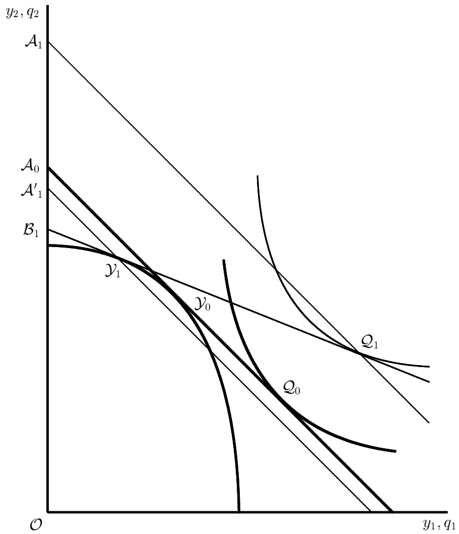
Figure 2: Endproducts Model — An improvement in the terms of trade increases real income (from \mathcal{O}A_0 to \mathcal{O}A_1 ), but it reduces real GDP (from \mathcal{O}A_0 to \mathcal{O}A'_1 )
