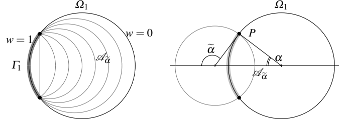
Fig. 2 Left: Level sets of w . Right: Geometric parametrization of a level set of w .
