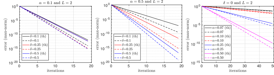
Fig. 6 Theoretical (solid line) and numerical (dashed line) convergences.
