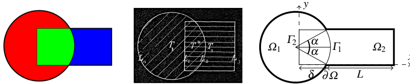
Fig. 1 Left: ddm logo. Center: Original drawing of Schwarz from 1870 [12]. Right: Geometric parametrization of the ddm logo.
