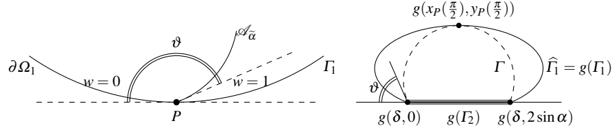
Fig. 3 Left: Geometry used in Lemma 1. Right: Geometric representation of Conjecture 1: the black solid curve represents \hat{\Gamma}_1 = g(\Gamma_1) and the black dashed arc of circle is \Gamma that passes through the points g(\delta, 0) , g(x_P(\frac{\pi}{2}), y_P(\frac{\pi}{2})) and g(\delta, 2\sin\alpha) . The set g(I_2) is [g(\delta, 0), g(\delta, 2\sin\alpha)] \times \{0\} and is marked in grey.
