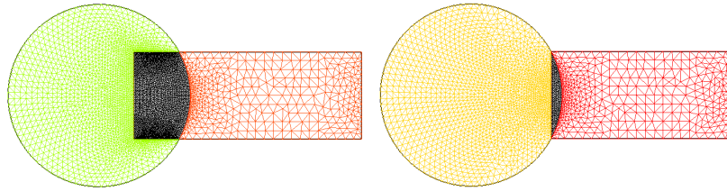
Fig. 5 Examples of finite element discretizations of the ddm logo obtained by Freefem. Left: \alpha = 0.5 , \delta = 0.5 and L = 2 . Right: \alpha = 0.5 , \delta = 0 and L = 2 .
