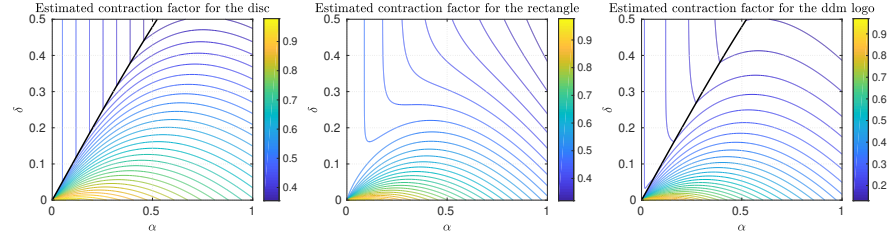
Fig. 4 Left: Values of \max_{\Gamma_2} v_1 as function of \alpha and \delta given in (6). Center: Estimate of \max_{\Gamma_1} v_2 given in (7). Right: Estimated convergence factor for the ddm logo given in (9).
