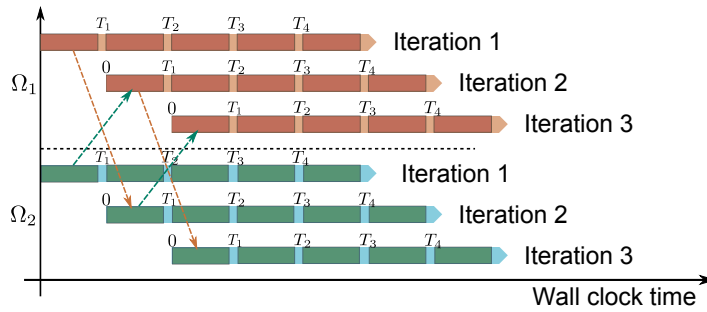
FIG. 7.8. Pipeline waveform relaxation method using six processors for two subdomains. Each bar represents a processor, with the darker color indicating time spent on numerical integration, and the lighter color indicating time spent on communication with neighboring subdomains. The T_i above the bars show which portion of the time window is being worked on at a particular instant in wall-clock time. The arrows indicate the transfer of interface data between subdomains.
