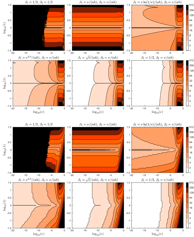
Fig. 1 Number of iterations for various \beta_1 and \beta_2 in 1D (top 6 panels) and 2D (bottom 6 panels).
