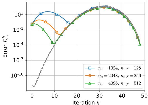
Fig. 4 Convergence of PARAREAL for the advection problem, using the SDIRK3-C6 space-time discretization, and varying the level of accuracy, with different number of mesh points n_x . Dashed gray lines represent E_\infty^k , using a zero initial condition and a random initial guess with unitary norm, scaled down to 1e^{-12} .
