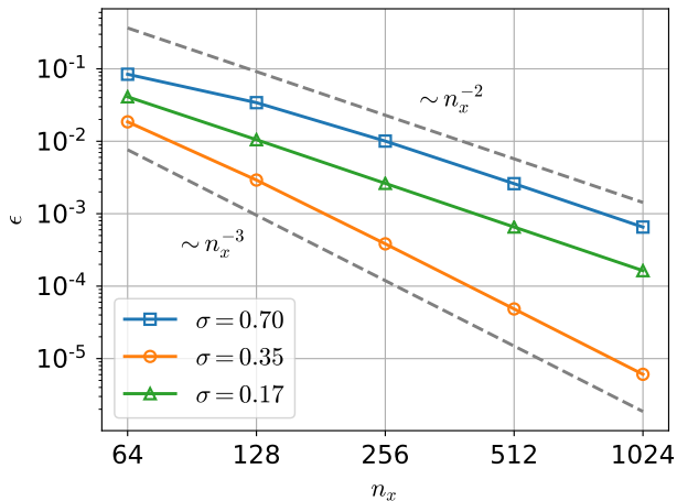
Fig. 2 Numerical error of SDIRK2-2 combined with a C2 space discretization, when varying the CFL number \sigma . Gaussian initial condition, and simulation during one temporal period of (1). Dashed lines represent error reduction of order 2 ( n_x^{-2} , top) and of order 3 ( n_x^{-3} , bottom).
