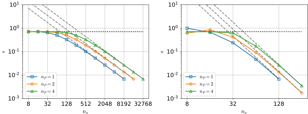
Fig. 1 Comparison of the theoretical error estimates in Theorem 1 to the effective numerical error. Left: Backward Euler and 6 th order centered finite differences, \kappa = 2 , A = 1 , \sigma = 1 . Right: SDIRK3 and 3 rd order upwind finite differences, \kappa = 1 , A = 1 , \sigma = 8 . The analytical error estimates are indicated by gray dashed lines, black dotted lines indicate the magnitude of the exact solution.
