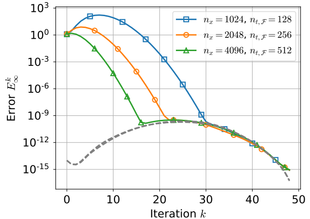
Fig. 3 Convergence of PARAREAL for the advection problem, using the BE-C6 space-time discretization, and varying the level of accuracy by using different numbers of mesh points n_x and n_{t,\mathcal{F}} . Dashed gray lines represent E_\infty^k , using a zero initial condition and a random initial guess with unitary norm, scaled down to 1e^{-14} .
