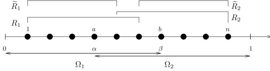
FIGURE 3.3. Definition of the \tilde{R}_j for a one dimensional example.
