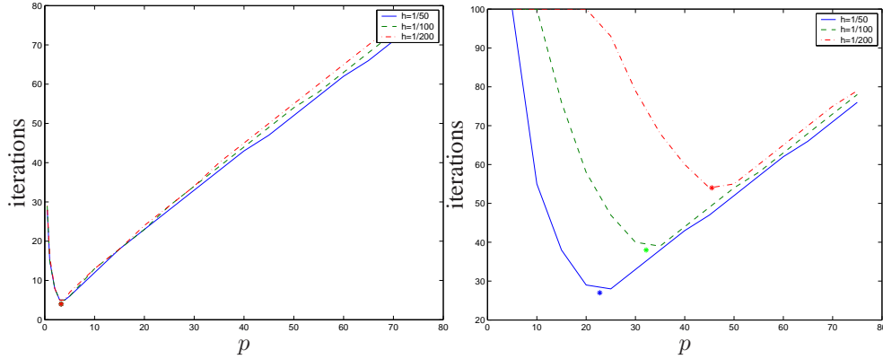
FIGURE 5.2. Using a zero initial guess and computing a smooth solution, the performance of the optimized Schwarz method does not seem to depend on h on the left. When, however, a random initial guess is used on the right, the dependence appears, as predicted by the theory.
