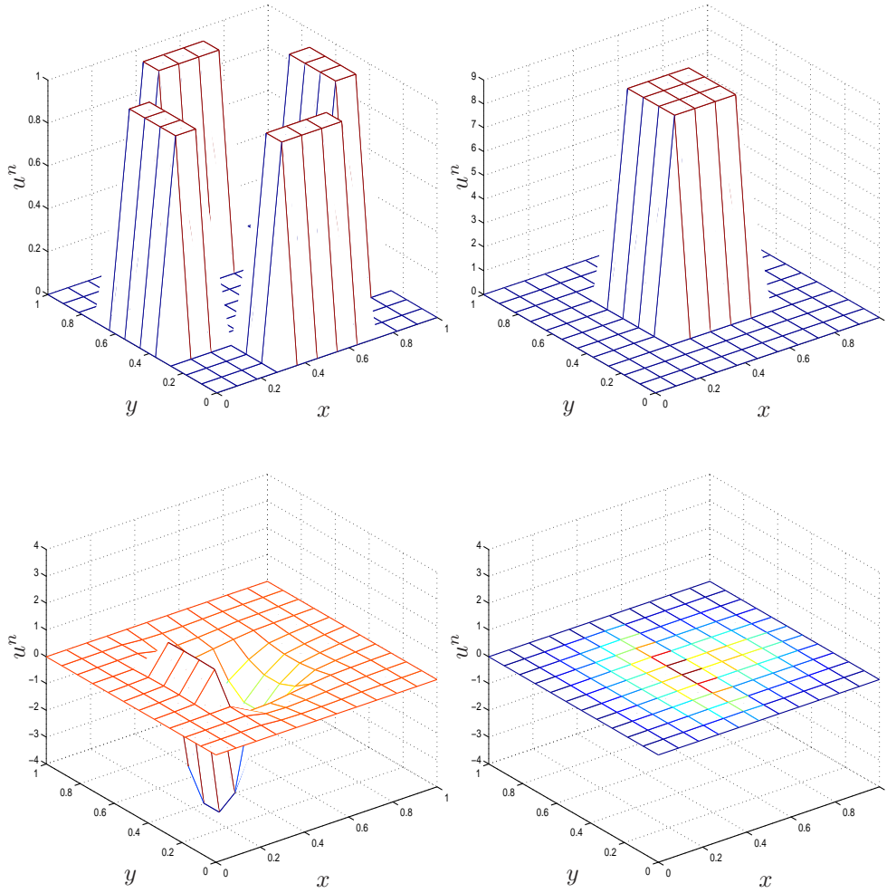
FIGURE 3.2. Error in the additive Schwarz method after two iterations, for various initial errors, and the result of Lions's parallel Schwarz method on the lower right for the same initial error as additive Schwarz on the lower left.
