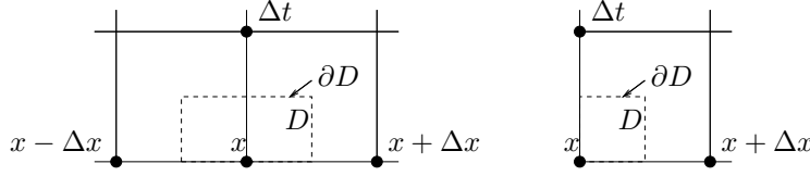
FIG. 5.2. Control volume of a grid point on the initial line and in a corner.
