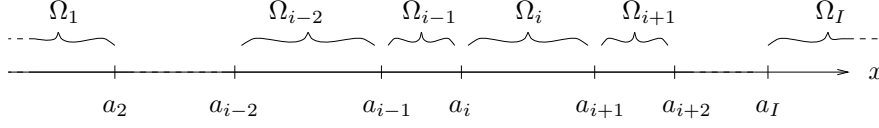
FIG. 2.1. Domain decomposition into I non-overlapping subdomains.
