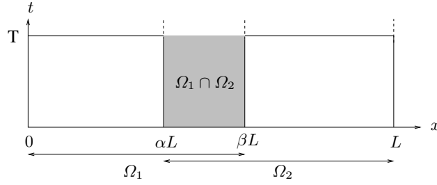
Fig. 1. Space-time domain decomposition.
