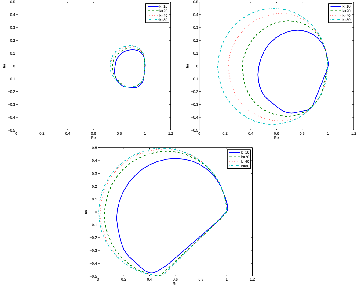
Fig. 1 The numerical range of \mathbf{A}_\varepsilon^{-1}\mathbf{A} , from top left to bottom for \varepsilon = k (top left), \varepsilon = k^{3/2} (top right), and \varepsilon = k^2 (bottom), k = 10, 20, 40, 80
