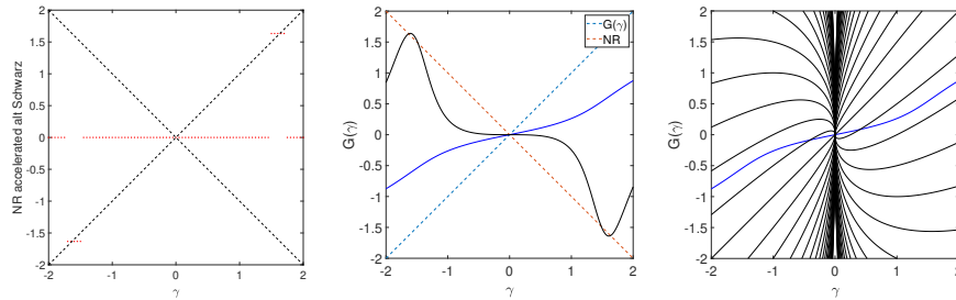
Fig. 3 Left: Results of Newton-Raphson accelerated alternating Schwarz as a function of initial condition in solving equation (1). The value of a is 3.6 and the subdomains are \Omega_1 = (-1, 0.2) and \Omega_2 = (-0.2, 1) . Middle: G(\gamma) and its Newton-Raphson acceleration. Right: G(\gamma) plotted with the geometry of the right of Figure 2.
