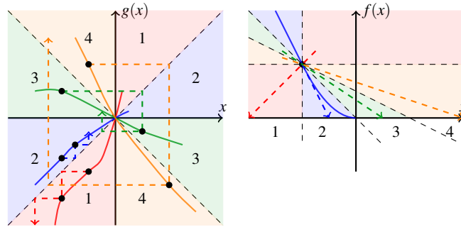
Fig. 1 Left: Behaviour of the fixed point iteration x_{n+1} = g(x_n) , where the origin is the fixed point, g(0) = 0 . Right: Regions of Newton-Raphson, x_{n+1} = x_n - f(x_n)/f'(x_n) , where the origin is the root, f(0) = 0 . The tangent line to f(x) can be traced from (x, f(x)) towards the line y = 0 . Where it lands on this line indicates which fixed point iteration behaviour occurs.
