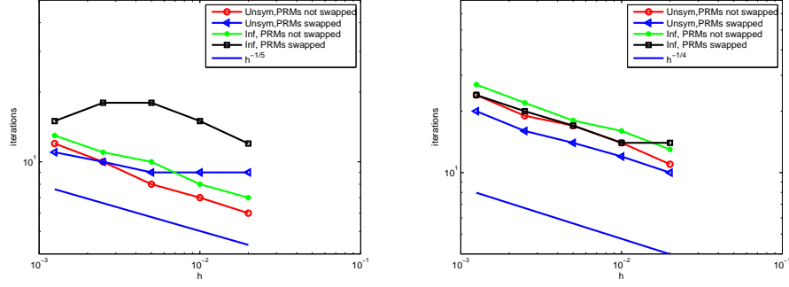
Fig. 1 Number of iterations required by the optimized Schwarz methods: overlapping case on the left, nonoverlapping case on the right.
