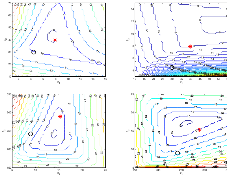
Fig. 2 Optimized parameters found by our analysis (*), as well as by the infinite domain decomposition analysis (o), compared to the performance of other values of the parameters: first row for the overlapping case, second row for the nonoverlapping case, with the parameters before parameter swapping in the left column and after swapping in the right column.
