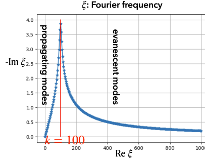
Fig. 1 Fourier frequencies from the Sturm-Liouville problem with C = \partial_n - ik for k = 100 .
