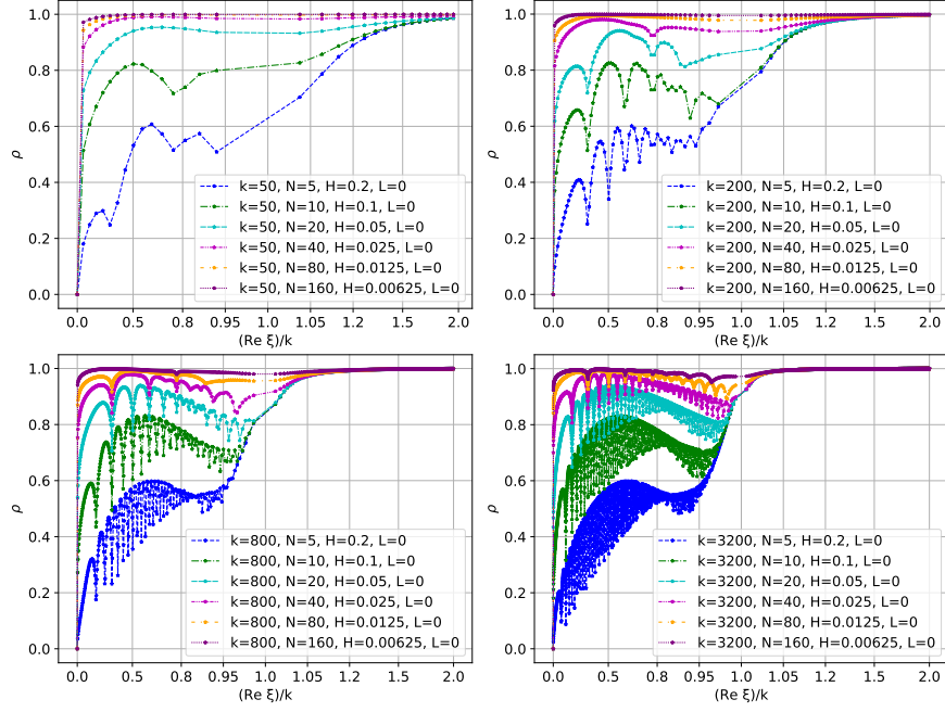
Fig. 2 \rho of Desprès' method for free space on [0, 1]^2 .
