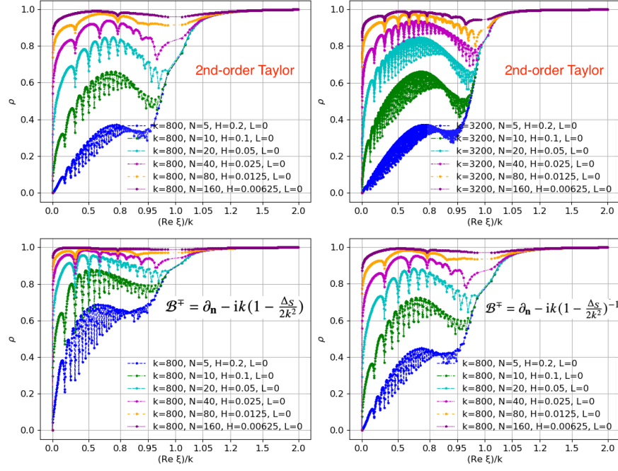
Fig. 9 \rho of Desprès' method plus a 2nd-order term for free space on [0, 1]^2 .
