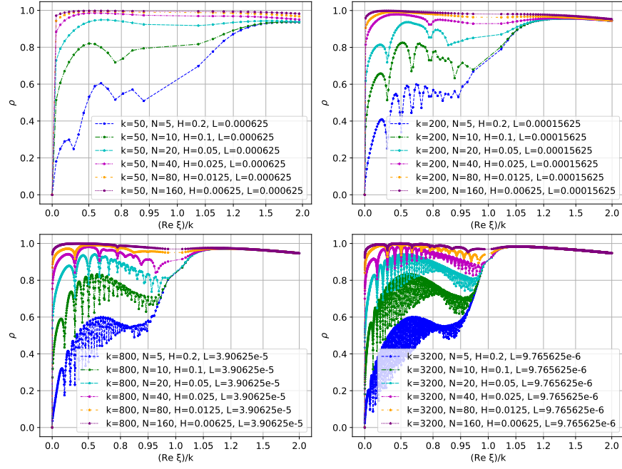
Fig. 4 \rho of Desprès' method plus L = \frac{1}{32k} overlap for free space on [-\frac{L}{2}, 1 + \frac{L}{2}] \times [0, 1] .
