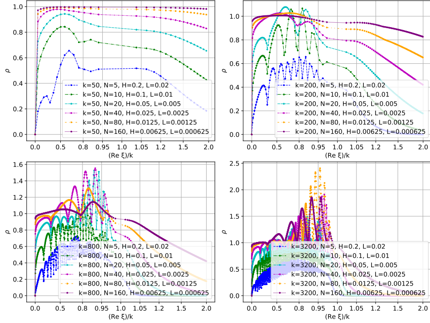
Fig. 3 \rho of Desprès' method plus L = \frac{H}{10} overlap for free space on [-\frac{L}{2}, 1 + \frac{L}{2}] \times [0, 1] .
