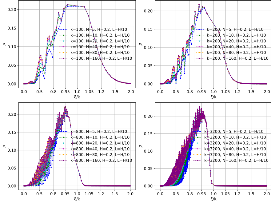
Fig. 6 \rho of Desprès' method plus L = \frac{H}{10} overlap in double sweep for free space on [-\frac{L}{2}, \frac{N}{5} + \frac{L}{2}] \times [0, 1] .
