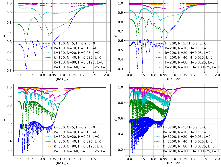
Fig. 7 \rho of Desprès' method with left/right Robin coeff. -ik(1 \pm 0.1i) for free space on [0, 1]^2 .
