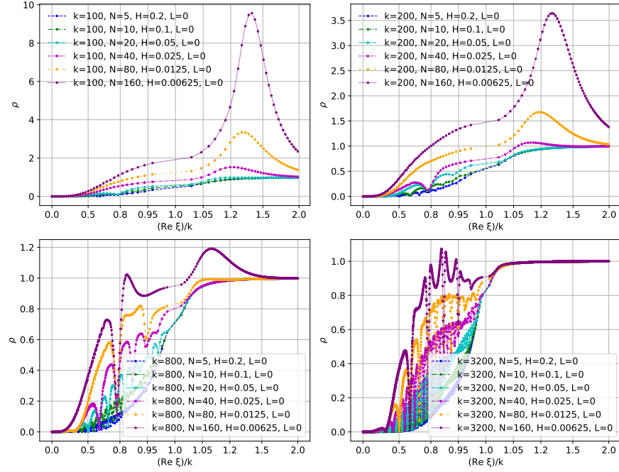
Fig. 5 \rho of Desprès' method in double sweep for free space on [0, 1]^2 .
