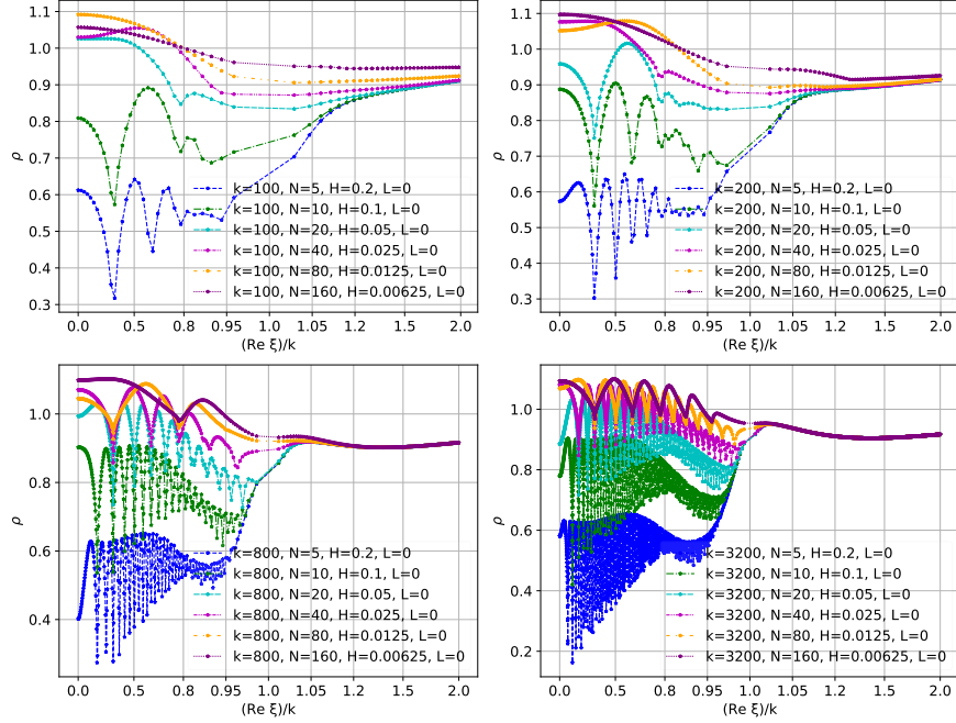
Fig. 8 \rho of Desprès' method with interface Robin coefficient -ik(1 + 0.1i) for free space on [0, 1]^2 .
