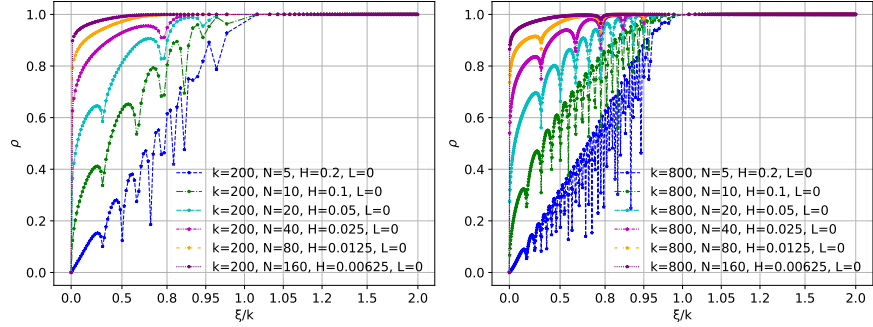
Fig. 10 \rho of Desprès' method with \mathcal{B}^\ddagger the 2nd-order Taylor for waveguide on [0, 1]^2 .
