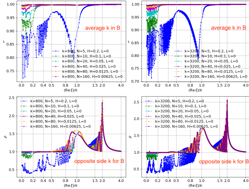
Fig. 11 \rho of Després' method on [0, 1]^2 with exterior wavenumber k & interior k/[1, 5, 0.5, 2, 1] .
