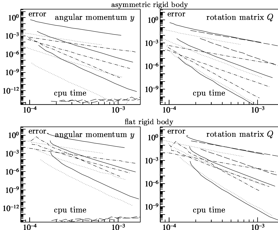
Figure 1: Work-precision diagrams for rigid body integrators: DMV, DMV4, DMV6 (solid lines), IMR2, IMR4, IMR6 (dotted lines), JEM2, JEM4 (dashed lines), SR2, SR4, SR6 (dashed-dotted lines).
