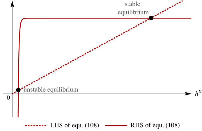
Figure A.1: Multiple steady states when the second inequality of (A2) is violated ( \varrho < 0 ). Parameters like in Tab. 1 except \psi = 1.9 .
