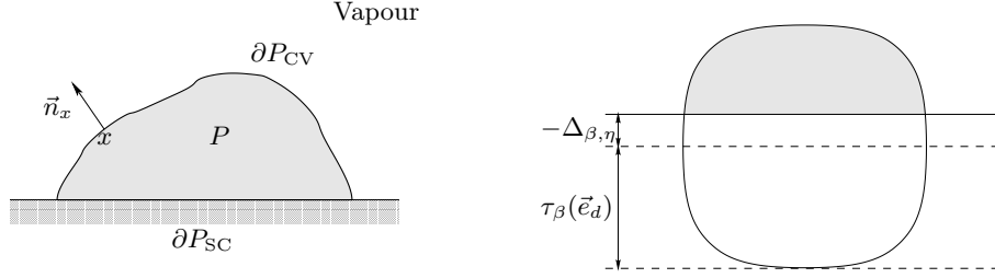
FIGURE 1. Left: The crystal P on the substrate. The boundary is decomposed into two pieces, corresponding to the crystal/vapor interface and the crystal/substrate interface. Right: The Winterbottom shape \mathcal{K}_{\beta,\eta} (shaded region) is obtained by intersecting the Wulff shape and the half-plane; on the picture \Delta_{\beta,\eta} is negative.
