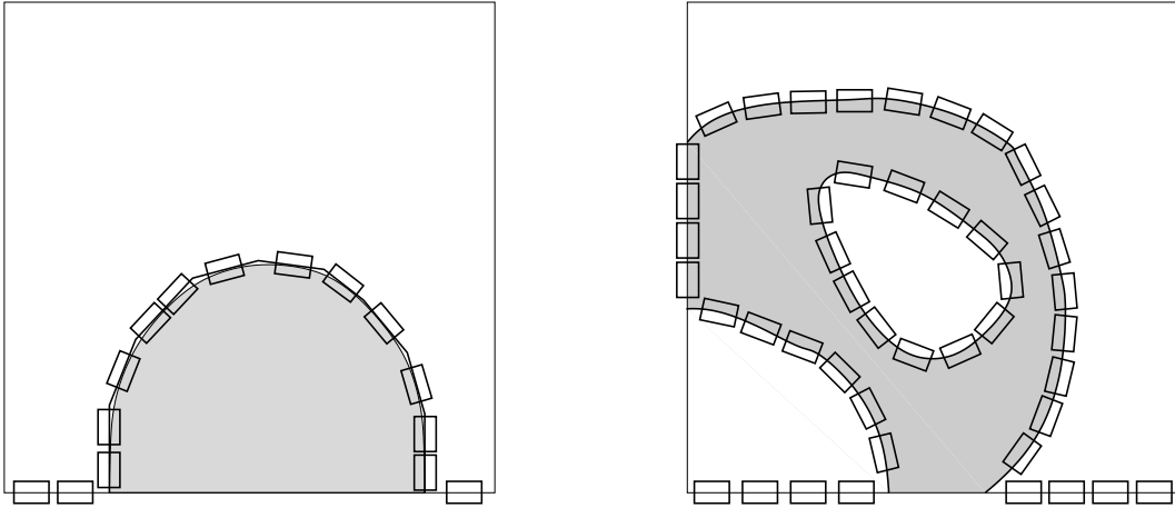
FIGURE 2. Left: The approximate Winterbottom shape \mathcal{K}_{\beta, \eta}^\delta(v(m)) and the boxes of Proposition 4.1. Right: A function v \in \text{BV}(\text{int}(\widehat{\mathbb{D}}, \{\pm 1\})) (the shaded area corresponds to v \equiv -1 ), and the boxes of Theorem 4.1.
