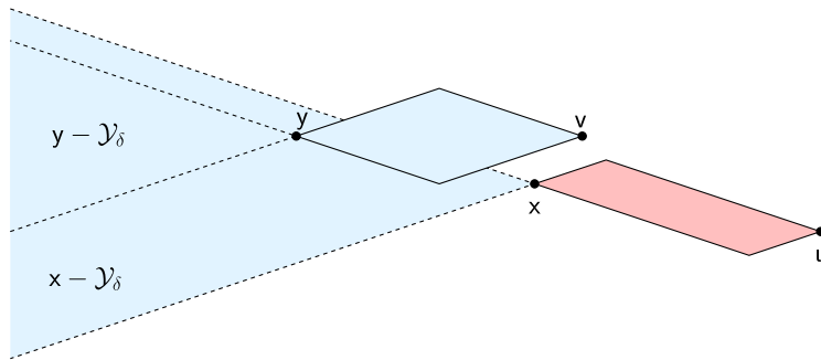
FIG. 2. With x, y, u, v as in the picture, the paths contributing to t_x^\omega t_y^\omega(q_{y,v}^\omega - \mathbf{q}_{y,v}) lie inside the blue region, while the paths contributing to q_{x,u}^\omega - \mathbf{q}_{x,u} lie inside the red region. These two quantities are thus independent (w.r.t. the disorder).
