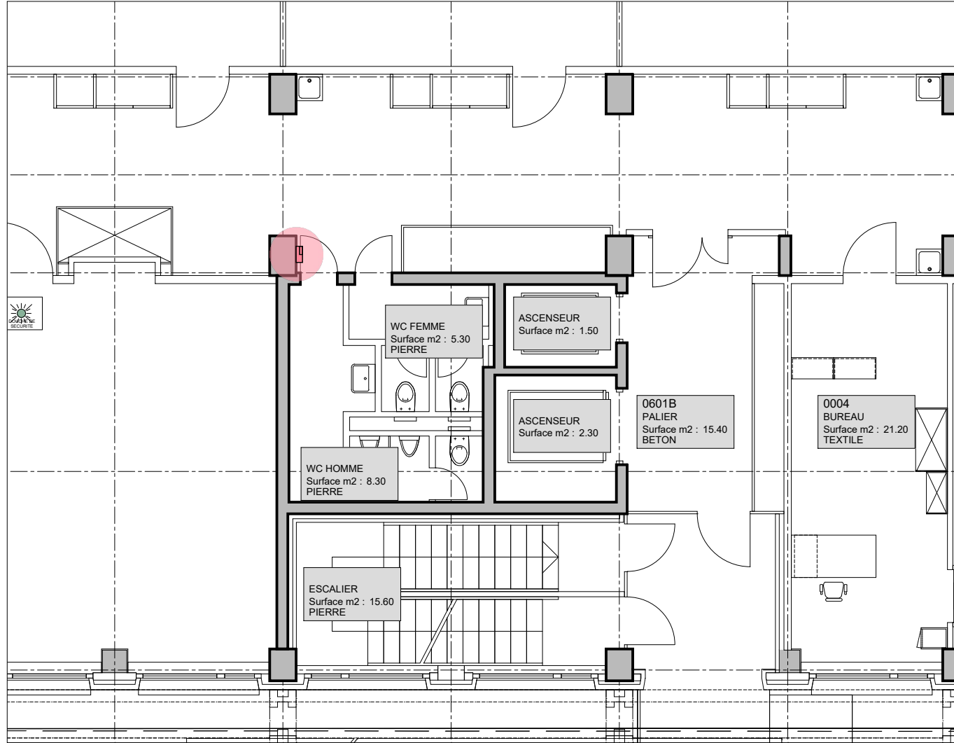
Plans 1:100
