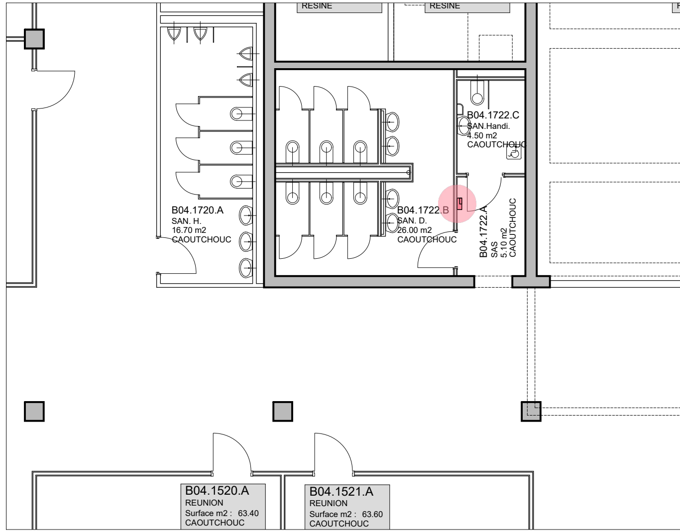
Plans 1:100
