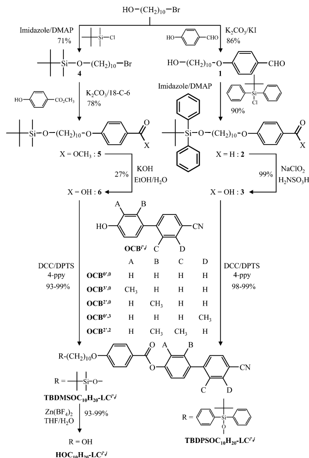
Scheme 2 Synthesis of calamitic cyanobiphenyls R-C 10 H 20 -LC i,j (DCC = N,N' -dicyclohexylcarbodiimide, DPTS = 4-[(dimethylamino)pyridinium]-4-toluenesulfonate, 4-ppy = 4-pyrrolidinopyridine, DMAP = 4-(dimethylamino)pyridine).
