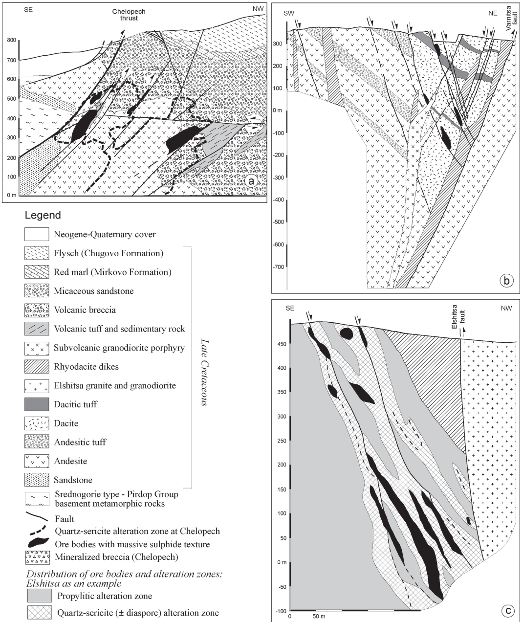
Fig. 4 (a) Cross sections of the Chelopech (after Chambefort, 2005), (b) Radka (after Popov and Popov, 1997; Tsonev et al., 2000b; Kouzmanov et al., 2002) and (c) Elshitsa deposits (after Chipchakova and Stefanov, 1974).
