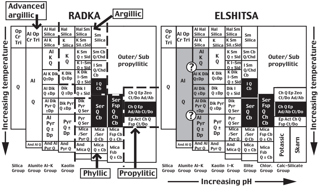
Fig. 5 Hydrothermal alteration assemblages described in the Chelopech (Petrunov, 1989, 1995; Georgieva et al., 2002), Krassen (Tsonev et al., 2000a), Radka (Tsonev et al., 2000b; Kouzmanov, 2001) and Elshitsa deposits (Radonova, 1967, 1970; Chipchakova and Stefanov, 1974; Dimitrov, 1985; Popov et al., 2000a; Kouzmanov, 2001) represented on diagrams after Corbett and Leach (Fig. 4.1, p. 71, 1998) showing the relative stability ranges of alteration mineral assemblages as a function of temperature and pH. The alteration zones (advanced argillic, argillic, phyllic, propylitic) defined in hydrothermal systems (Corbett and Leach, p. 73, 1998) are only represented for the Radka deposit, for the sake of clarity. The characteristic alteration assemblages of each deposit are highlighted with white letters on a black background. For Elshitsa, there is an additional grey background with question marks, because Dimitrov (1985) reports an alunite facies without mentioning the other alteration minerals present in the same facies, therefore the alteration assemblage remains uncertain. Ab—albite; Act—actinolite; Ad—adularia; Al—alunite; And—andalusite; Bio—biotite; Cb—carbonate; Ch—chlorite; Chab—chabazite; Chd—chalcedony; Ch—chlorite; Cr—cristobalite; Ct—calcite; Do—dolomite; Dik—dickite; Dp—diaspore; Ep—epidote; Fsp—feldspar; Hal—halloysite; I—illite; K—kaolinite; Op—opaline silica; Pyr—pyrophyllite; Q—quartz; Ser—sericite; Sid—siderite; Sm—smectite; Tri—tridymite.
