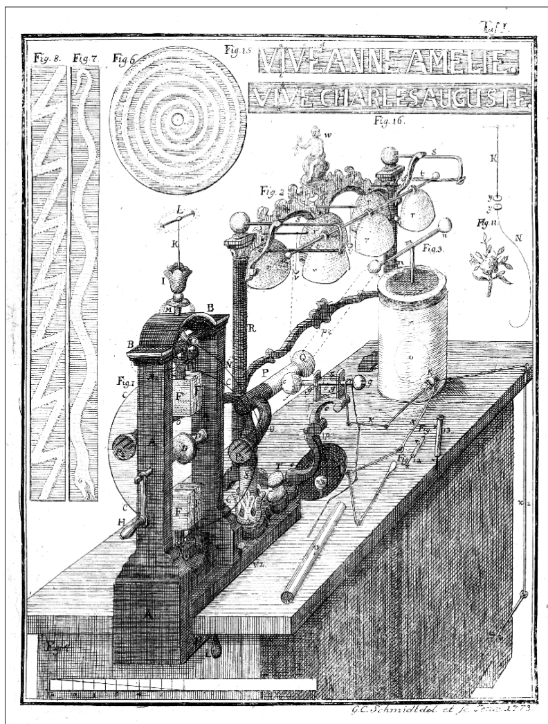
Fig. 3. Plate I from Schmidt (1773), showing the electrical machine and additional equipment.
