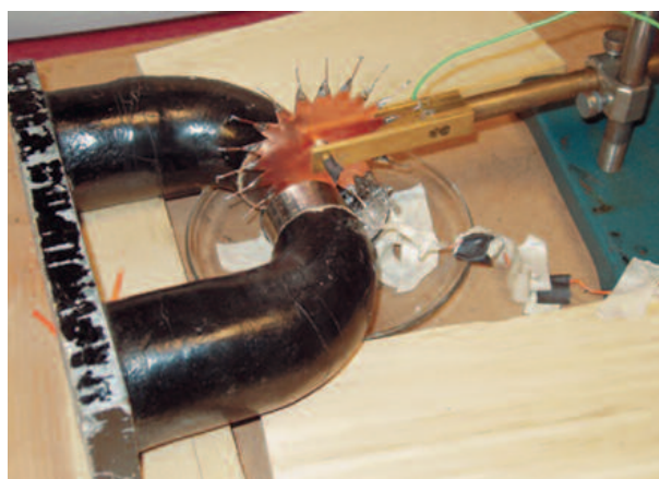
Fig. 9. Arrangement of magnet, my star wheel, galinstan puddle, and connections to power supply (not shown) resulting in motion.
