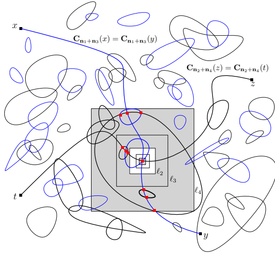
Figure 1: The two (duplicated)-currents \mathbf{n}_1 + \mathbf{n}_3 and \mathbf{n}_2 + \mathbf{n}_4 in blue and black respectively. The clusters of x (or equivalently y ) in \mathbf{n}_1 + \mathbf{n}_3 and z (or equivalently t ) in \mathbf{n}_2 + \mathbf{n}_4 are depicted in bold. The red vertices are the elements of the intersection \mathcal{I} . We illustrated the annuli around one element, denoted u , of \mathcal{I} and draw them in gray when an intersection occurs. Here, we therefore have M_u(\mathcal{I}; \mathcal{L}, 5) = 3 since three annuli contain an intersection.
