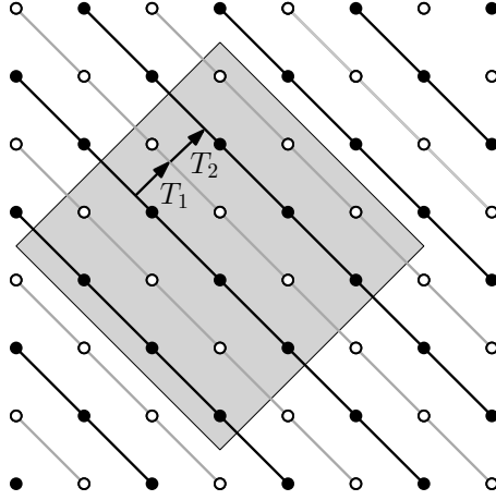
Figure 3: The split of Z^2 into even and odd sub-lattices and their stratification into intertwined diagonal hyperplanes. The partition function of (-L, L]^2 with rotated-periodic boundary condition can be written as Z_{2L} = \text{tr}(T_2 T_1)^L , with T_j a pair of conjugate mapping between the Hilbert spaces of the even and the odd hyperplanes. The product T_2 T_1 = T_1^* T_1 provides the even subgraph's transfer matrix in one of this graph's principal directions.
