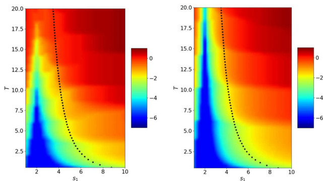
Fig. 17 Logarithm of the error in the wave domain after 6 iterations depending on s_1 and T when s_2 = -s_1 and |l_w| = |l_h| = 2 and 4 (from left to right). The crosses represent the theoretical values s^* from Theorem 2
