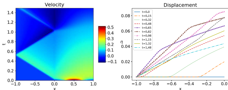
Fig. 9 As in Fig. 8, but now with initial data supported in the heat domain
