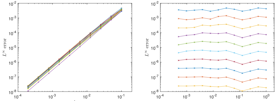
Figure 4: Method with uniform order 2 for multiplicity p = 1 . Error as a function of h for \varepsilon \in \{2^{-k}, k = 0, \dots, 11\} (left) and error as a function of \varepsilon for h \in \{0.1/2^k, k = 0, \dots, 9\} (right).
